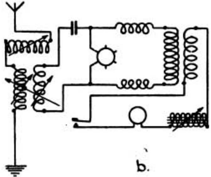
SAME CIRCUIT USING SYMBOLS AS SUGGESTED
