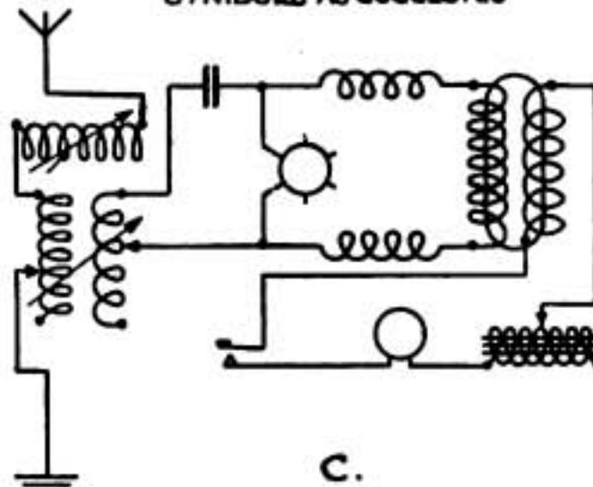
SAME CIRCUIT USING SYMBOLS AS SUGGESTED
