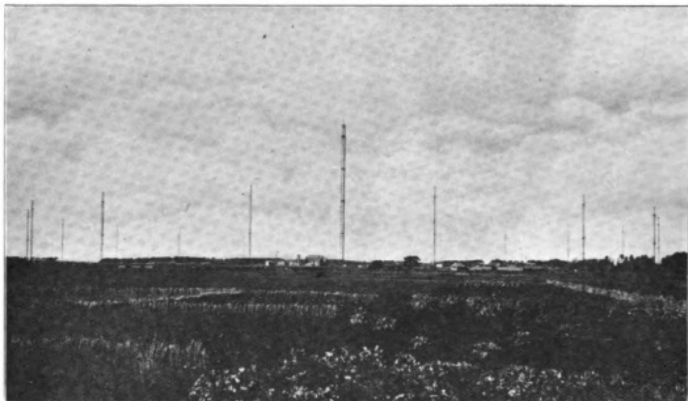
THE FUNABASHI STATION, SHOWING THE 650 FEET CENTRAL MAST AND THE EIGHTEEN SURROUNDING MASTS EACH 260 FEET HIGH.
