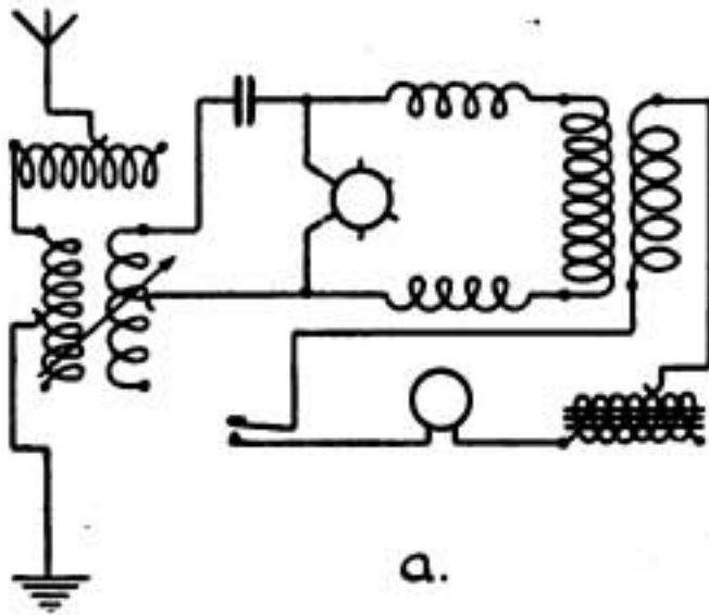
TRANSMITTER CIRCUIT AS SHOWN
